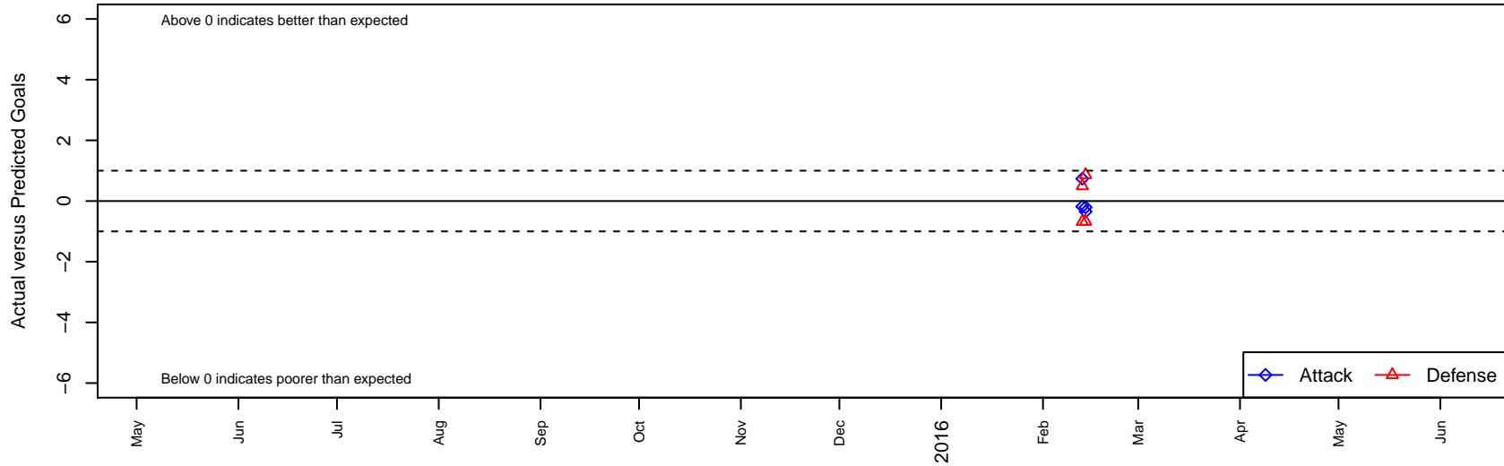
Slammers Orange –Unk B97 Dots are actual minus expected GF (blue circles) and GA (red triangles). Blue line is smoothed change in attack strength. Red is smoothed change in defense strength.
